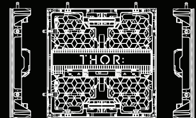
500mm x 500mm x 88mm Straight Latches
